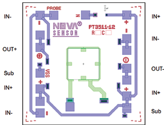
PT3511 Wire Bond Diagram
